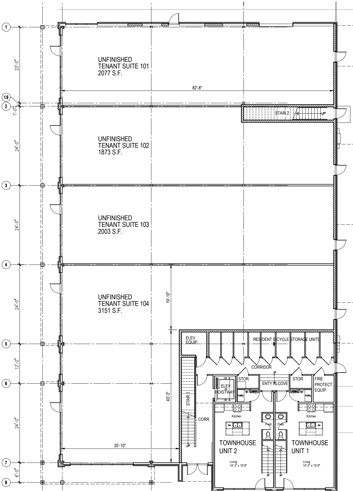
1st Floor Plan NOT TO SCALE
